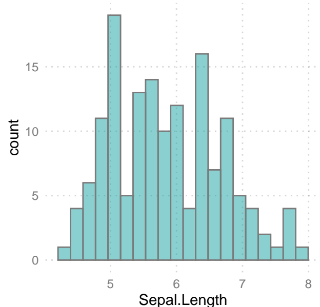
Distribution of Sepal Length (iris)
