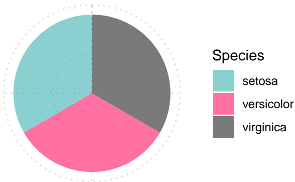
Species Composition
